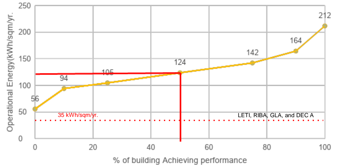
Operational Energy from Electric only Student Accommodations
